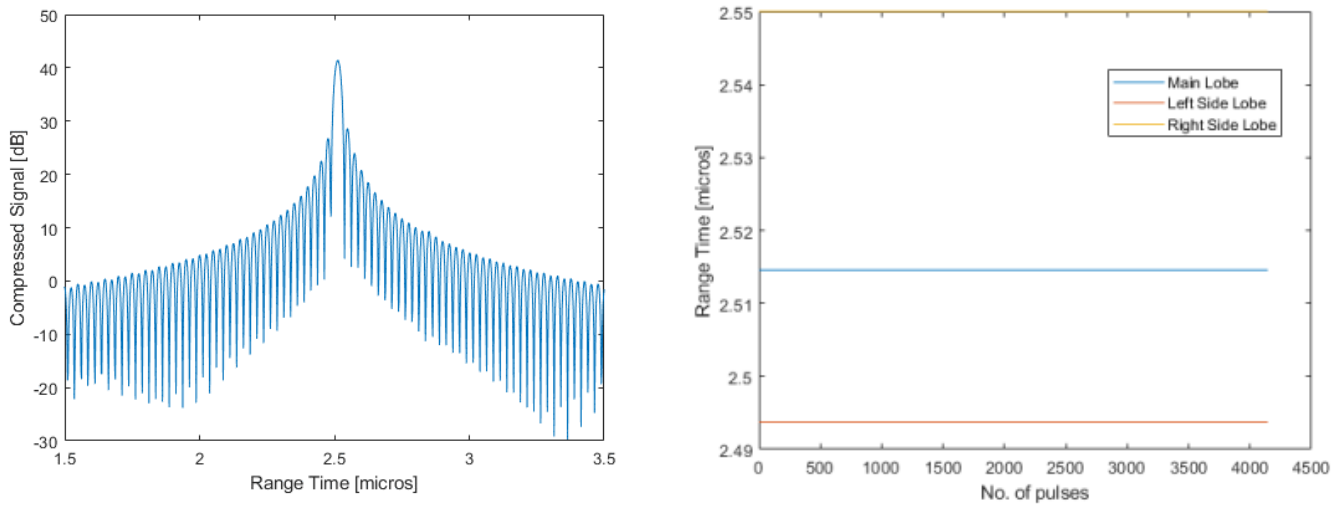
Figure 2-4: Test nr. 5 results; Left: compressed signal zoomed on the maximum value. Right: Compressed signal peak position throughout the test
