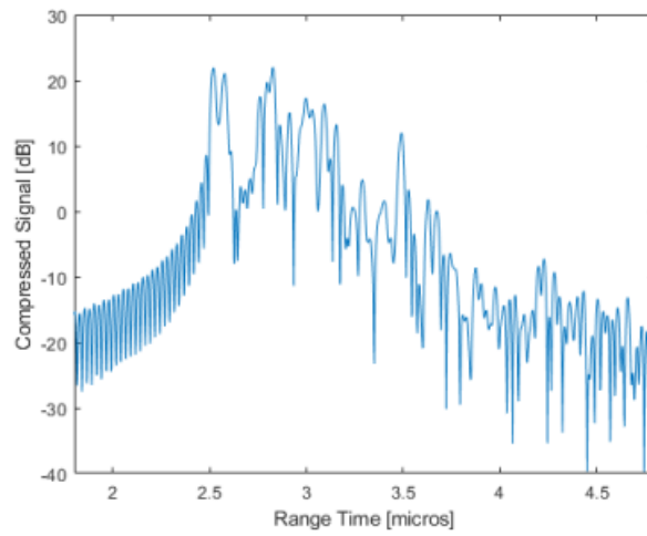
Figure 2-5: Compressed signal with a zoom around maximum value (test nr. 6)
