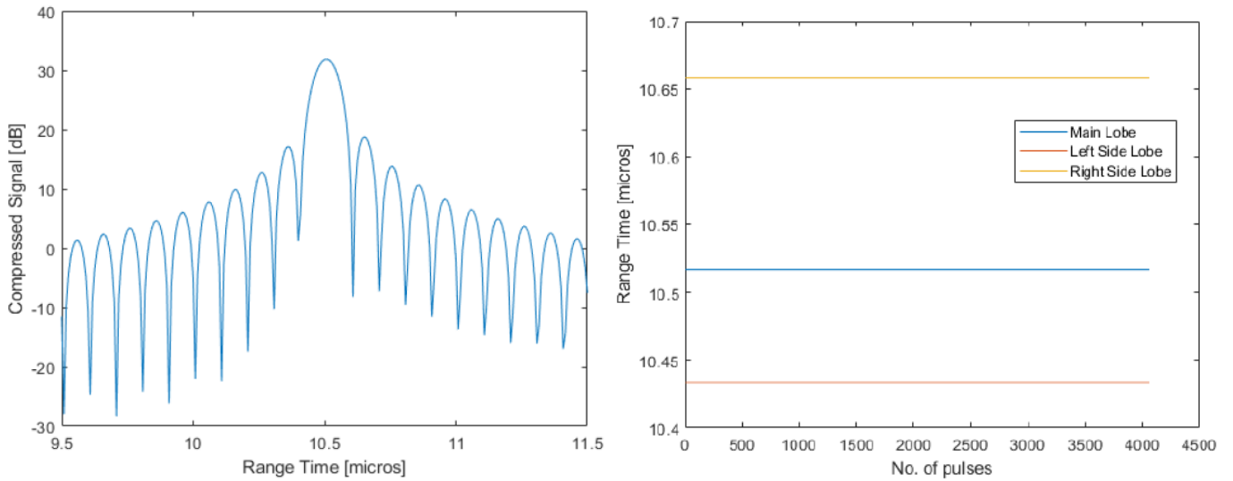
Figure 2-2: Test nr. 2 results; Left: compressed signal zoomed on the maximum value. Right: Compressed signal peak position throughout the test
