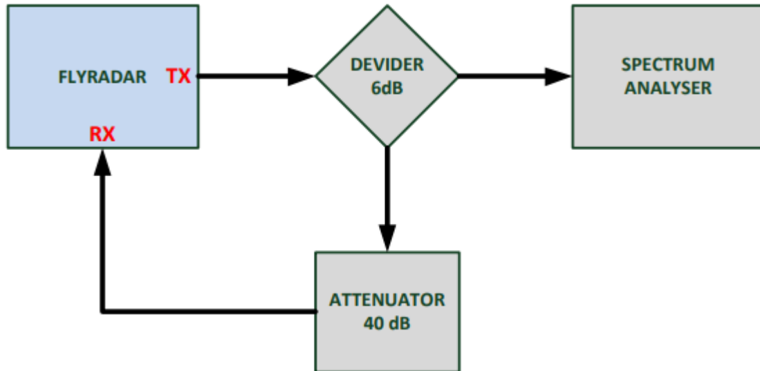
Figure 2-1: Test Configuration 2 (extracted from Co.Ri.S.T.A test report).
