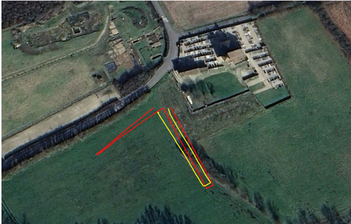
Figure 4-6– Field test tracks: HH in red and VV in azimuth.
