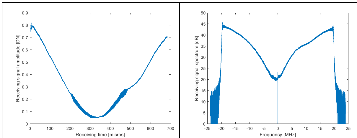
Figure 4-9– Field test, VV configuration: received and averaged signal in time (left) and frequency (right) domains.
