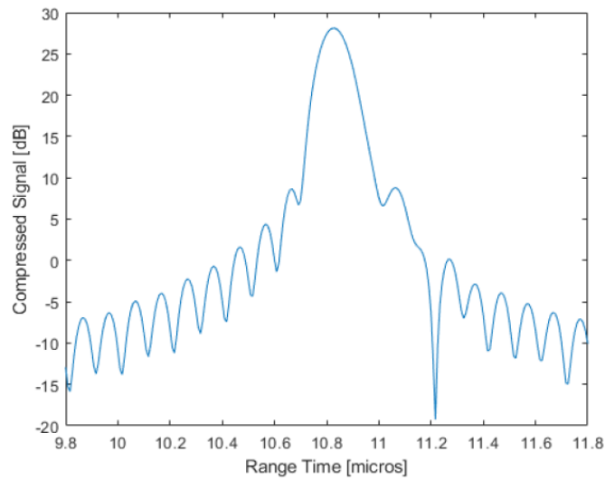
Figure 2-3 Compressed signal zoomed on the maximum value (Test nr. 3)
