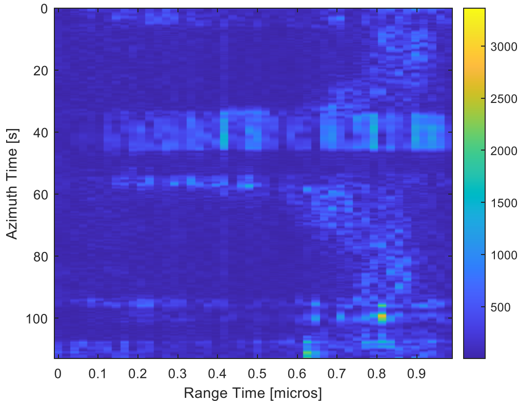
Figure 4-10– Field test, VV configuration: unfocused image.
