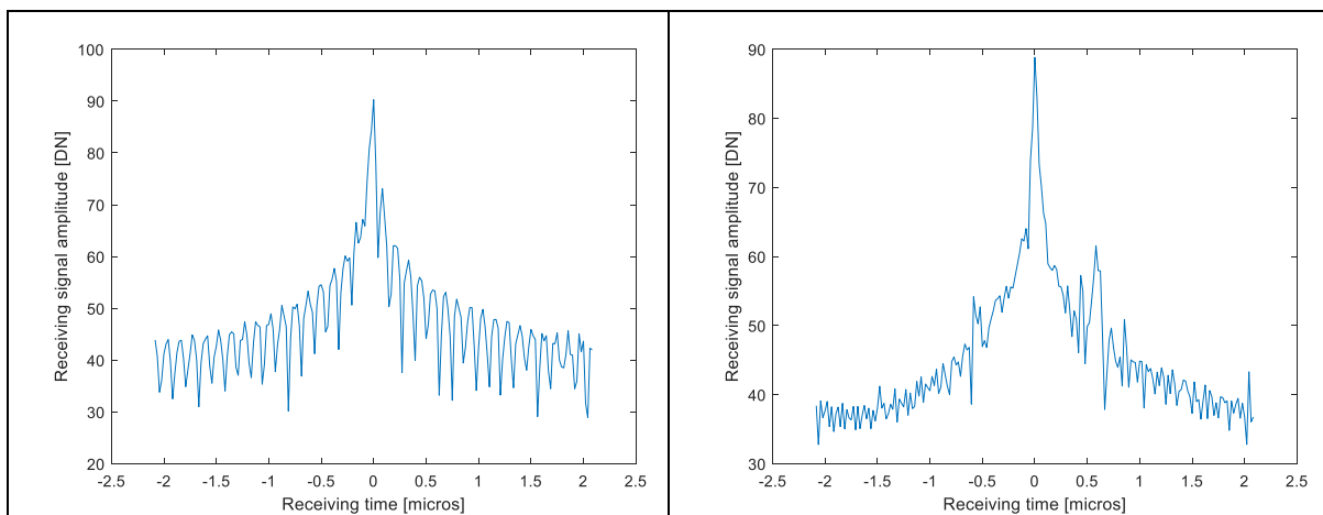
Figure 4-4– Laboratory test, VV configuration, compressed and averaged signal: peak value (left) and received signal amplitude (right).
