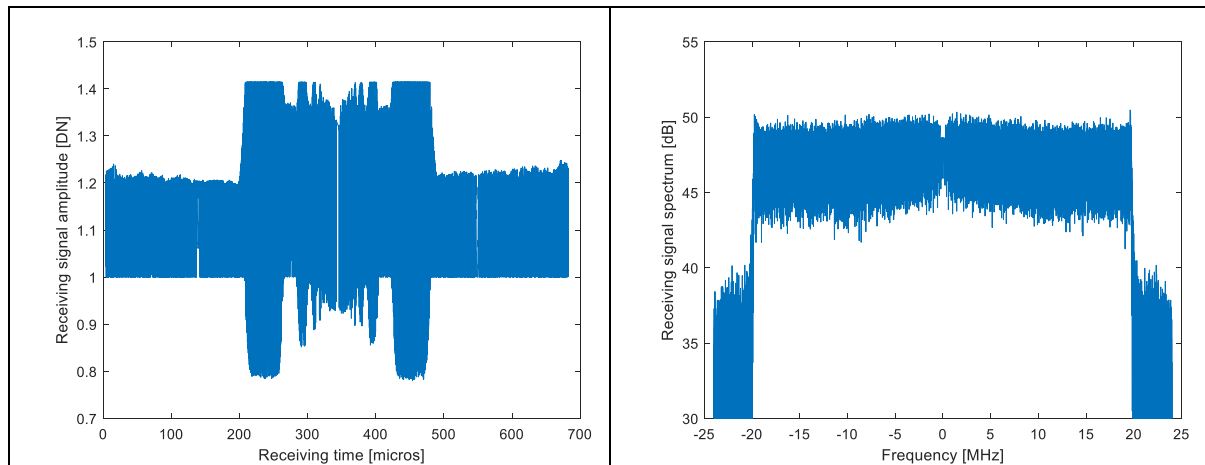
Figure 4-1– Laboratory test, HH configuration: received and averaged signal in time (left) and frequency (right) domains.
